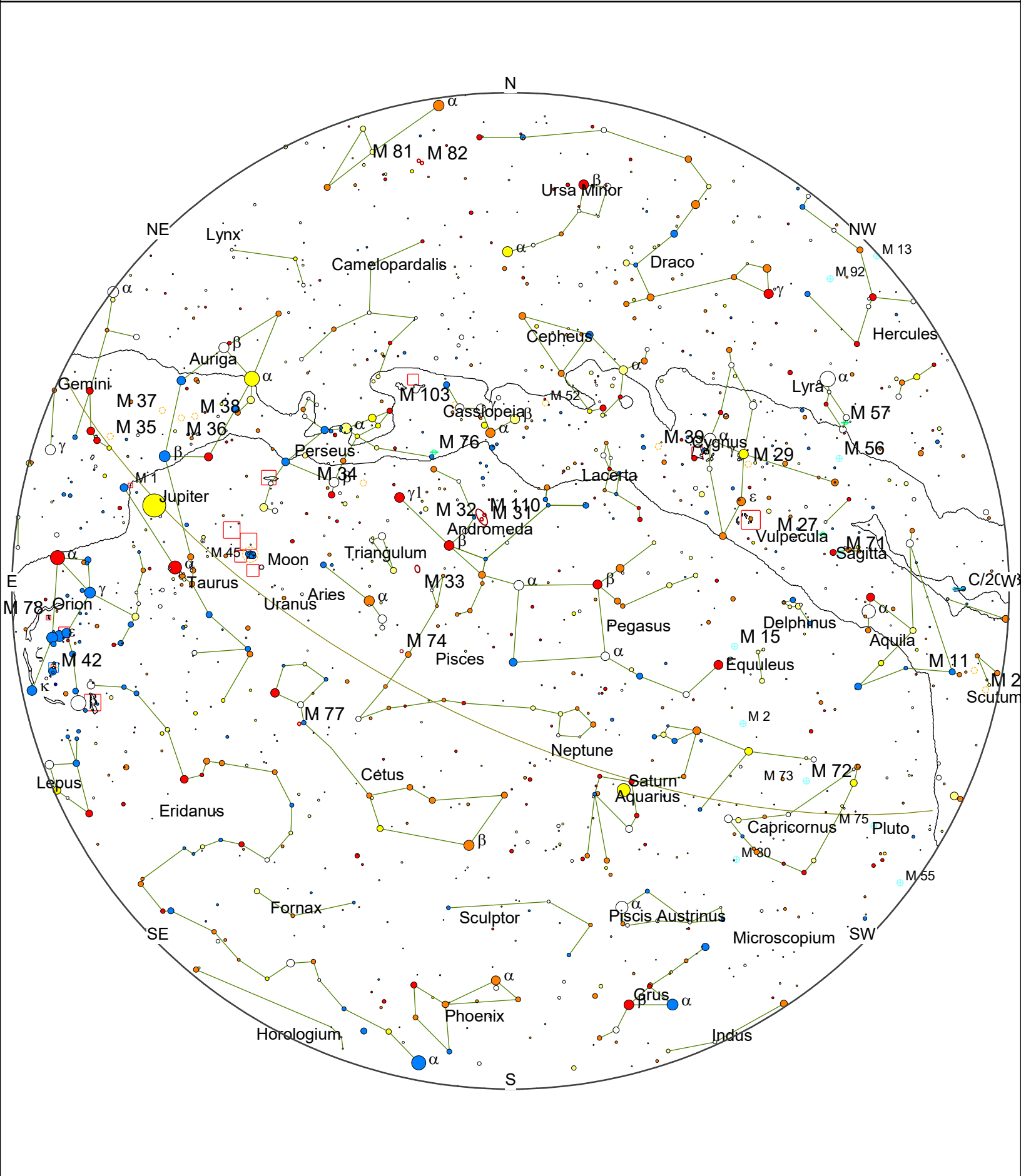
Alt/Az coord. ARC, Apparent, Broadmoor Astro, 2024-11-15, 21h00m00s (EST), Mag:5.5/6.0,100.0", FOV:+184°19'12"
